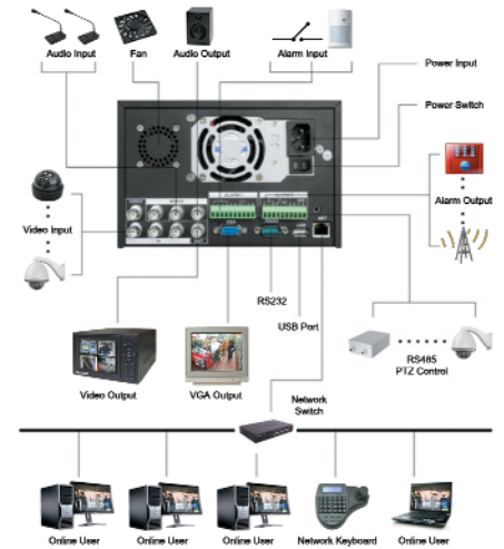
Connection Diagram
